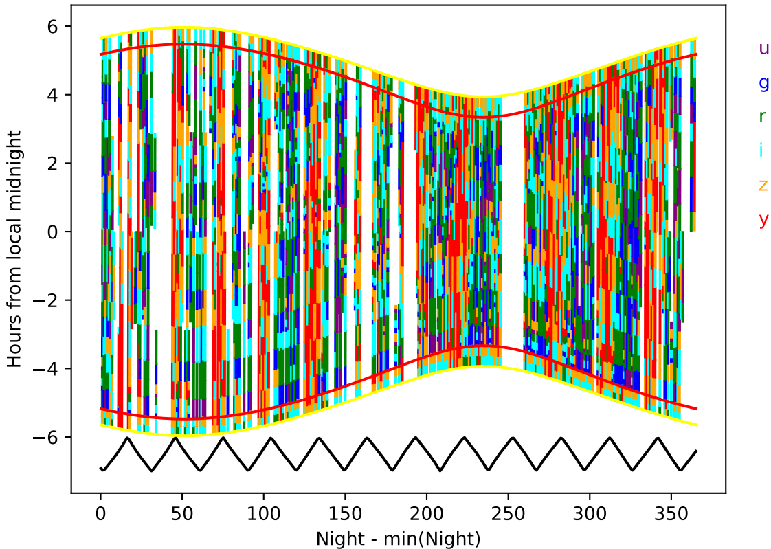
ddf_acor_sf15_lsf20_lsr50_v3.4_10yrs year 5-6: Hourglass
