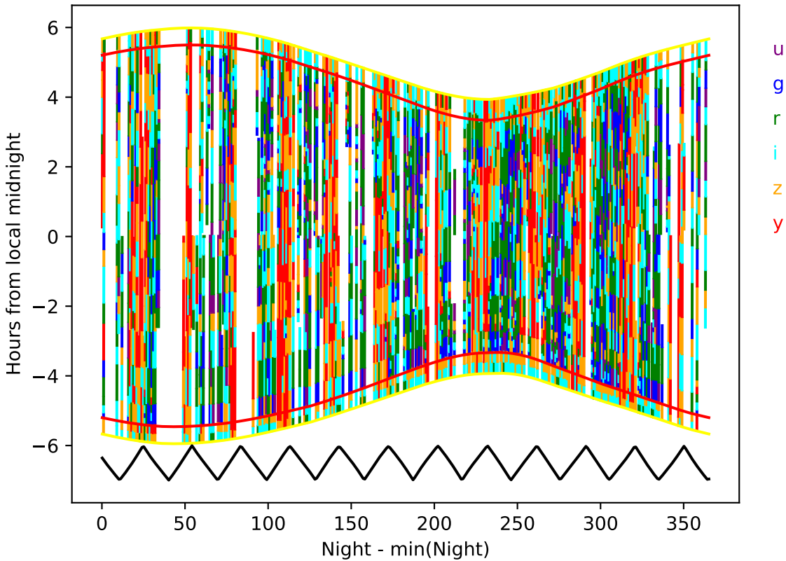
ddf_acor_sf15_lsf20_lsr50_v3.4_10yrs year 4-5: Hourglass
