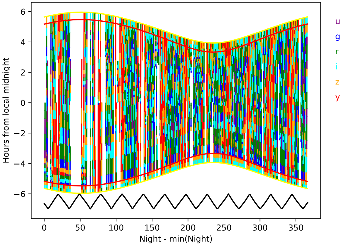
ddf_acor_sf15_lsf20_lsr50_v3.4_10yrs year 2-3: Hourglass
