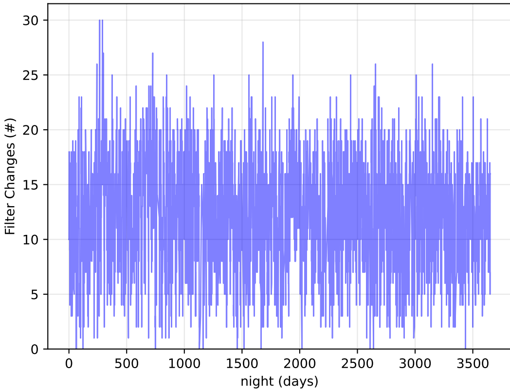
ddf_acor_sf15_lsf20_lsr50_v3.4_10yrs : Filter Changes
