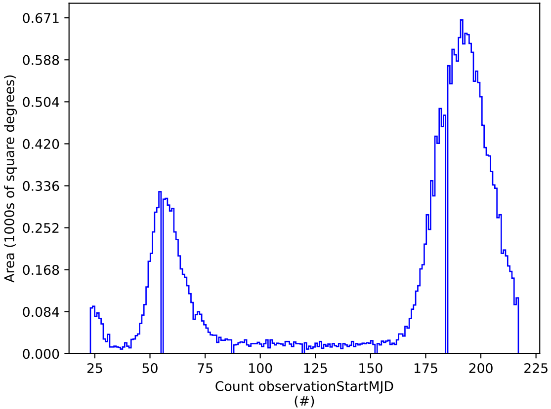
ddf_acor_sf15_lsf20_lsr50_v3.4_10yrs i: Count observationStartMJD
