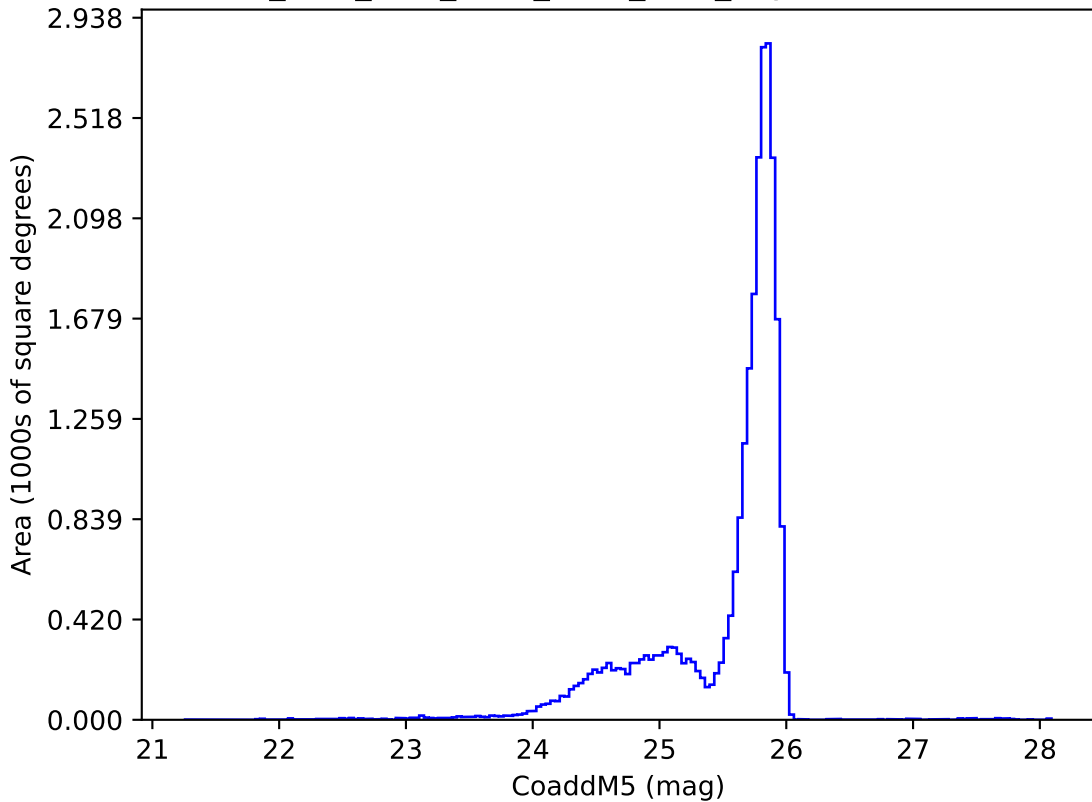
ddf_acor_sf15_lsf20_lsr50_v3.4_10yrs z: CoaddM5
