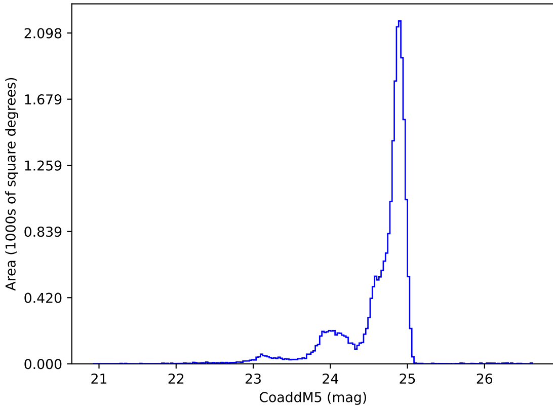
ddf_acor_sf15_lsf20_lsr50_v3.4_10yrs y: CoaddM5
