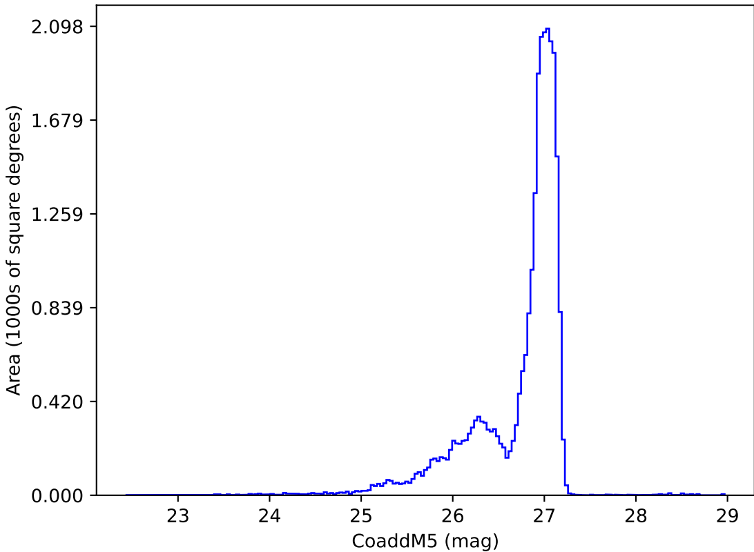
ddf_acor_sf15_lsf20_lsr50_v3.4_10yrs r: CoaddM5
