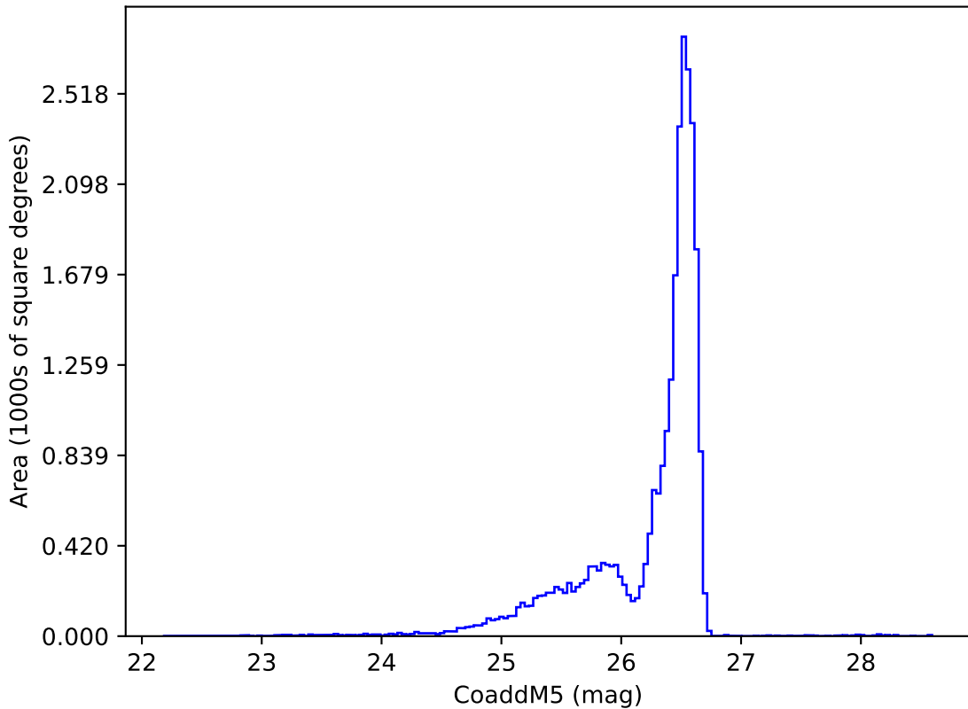
ddf_acor_sf15_lsf20_lsr50_v3.4_10yrs i: CoaddM5
