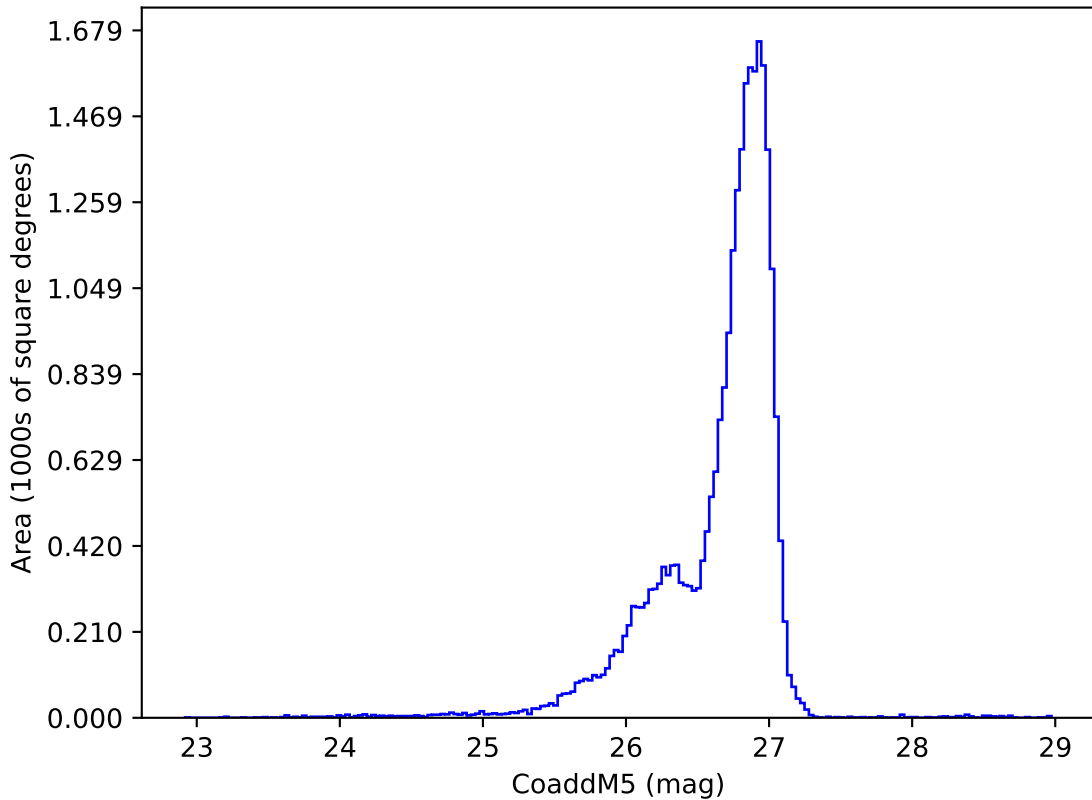
ddf_acor_sf15_lsf20_lsr50_v3.4_10yrs g: CoaddM5
