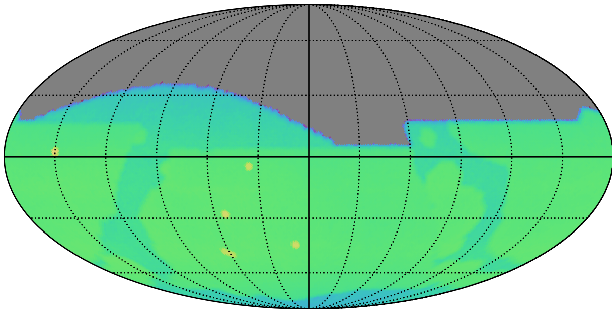
ddf_acor_sf15_lsf20_lsr50_v3.4_10yrs : CoaddM5
