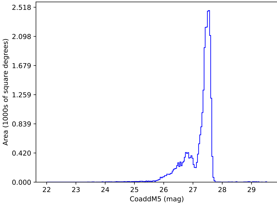
ddf_acor_sf15_lsf20_lsr50_v3.4_10yrs : CoaddM5
