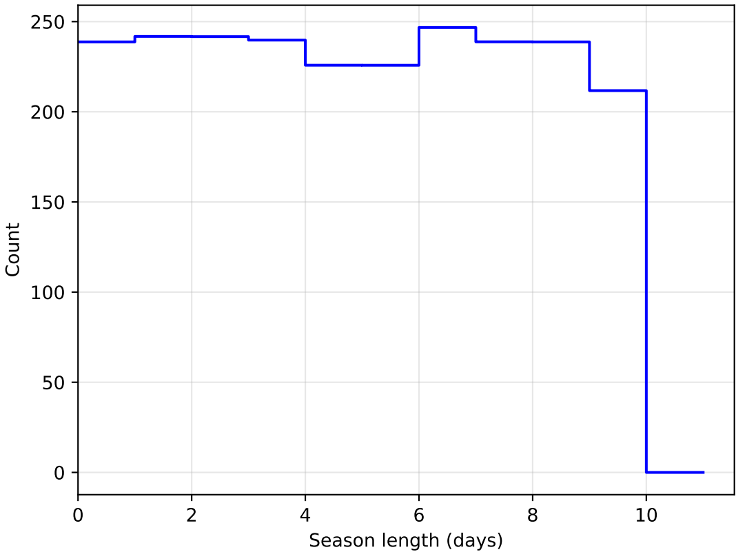
ddf_acor_sf15_lsf20_lsr50_v3.4_10yrs DD:EDFS all bands: SeasonLength
