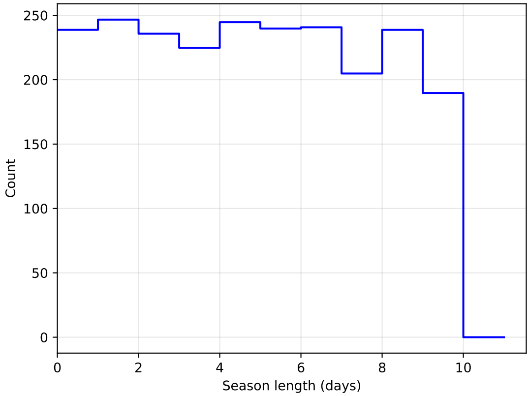
ddf_acor_sf15_lsf20_lsr50_v3.4_10yrs DD:ECDFS all bands: SeasonLength
