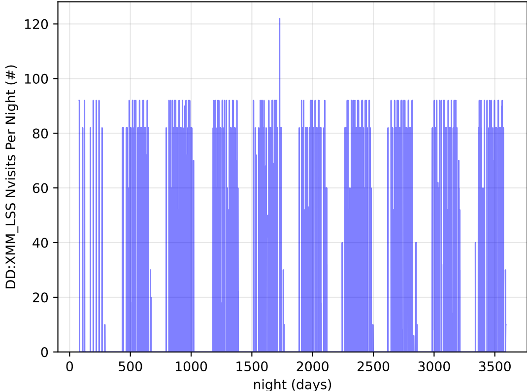
ddf_acor_sf15_lsf20_lsr50_v3.4_10yrs all bands: DD:XMM_LSS Nvisits Per Night
