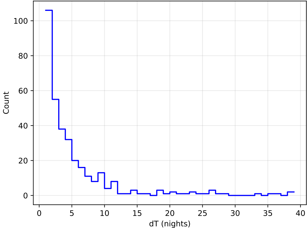
ddf_acor_sf15_lsf20_lsr50_v3.4_10yrs all bands: DD:WFD Delta Nights Histogram
