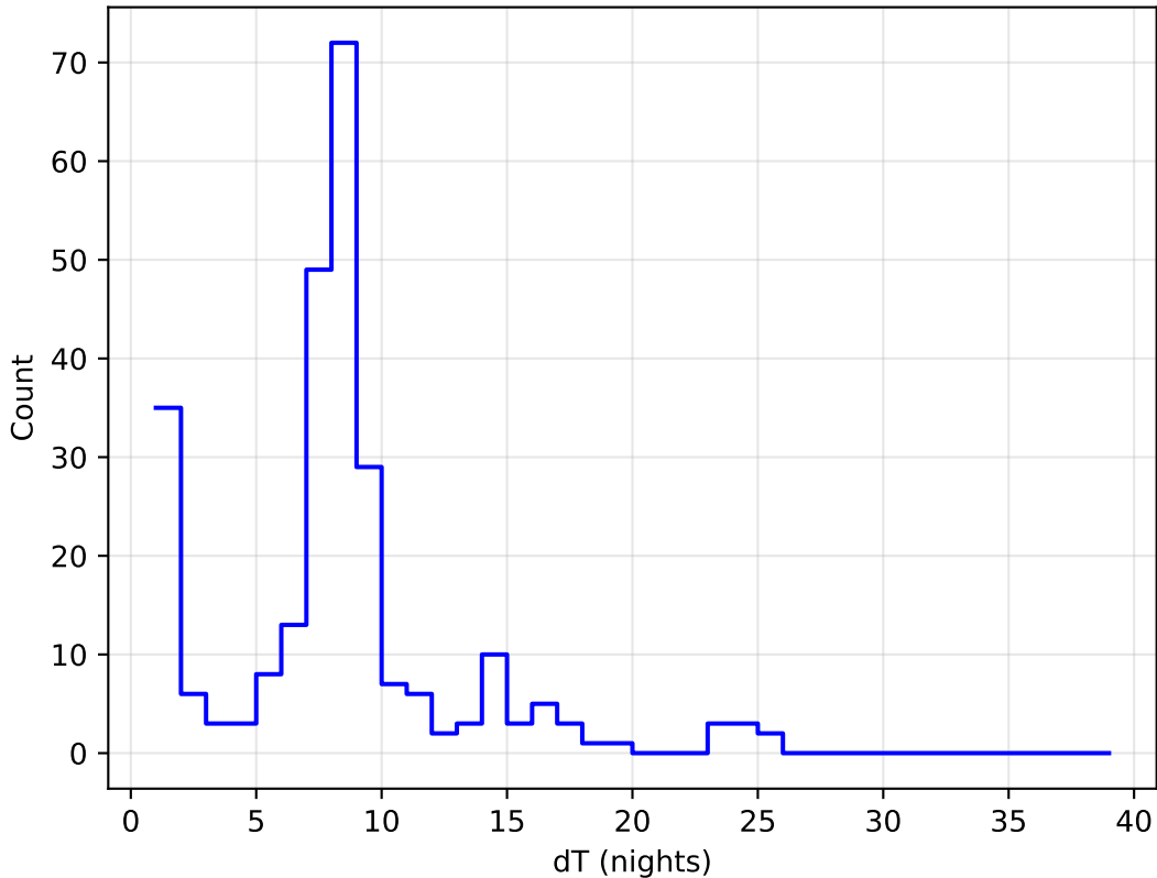
ddf_acor_sf15_lsf20_lsr50_v3.4_10yrs all bands: DD:ELAISS1 Delta Nights Histogram
