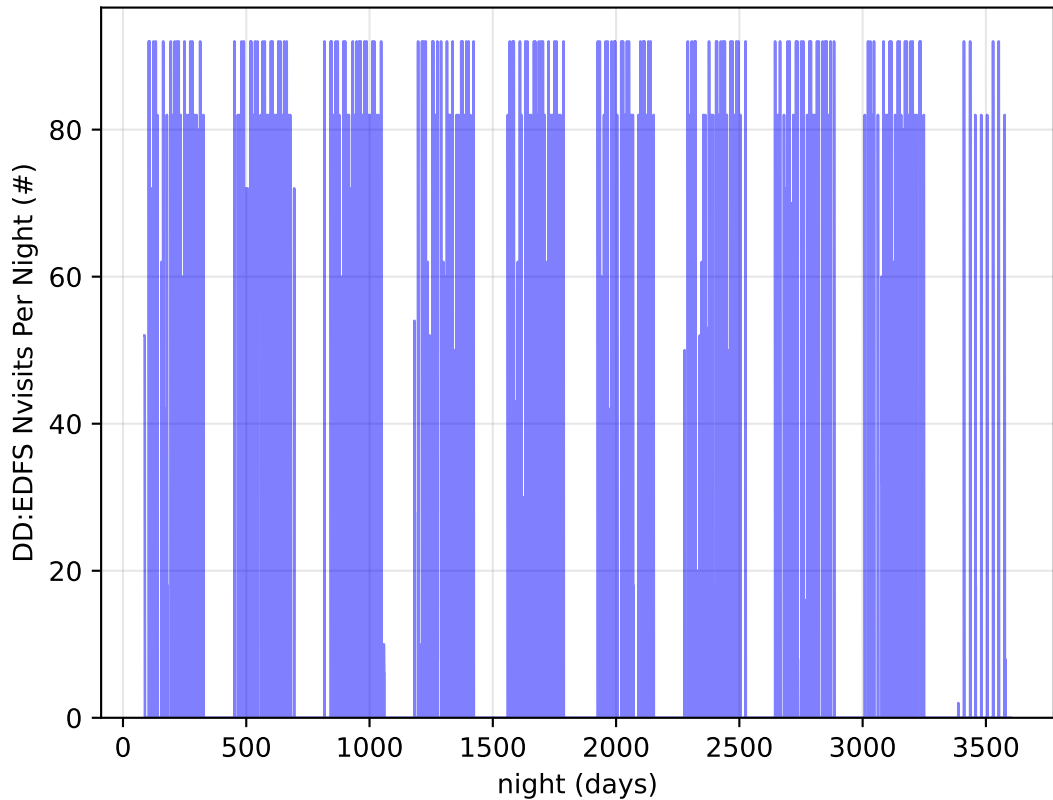
ddf_acor_sf15_lsf20_lsr50_v3.4_10yrs all bands: DD:EDFS Nvisits Per Night
