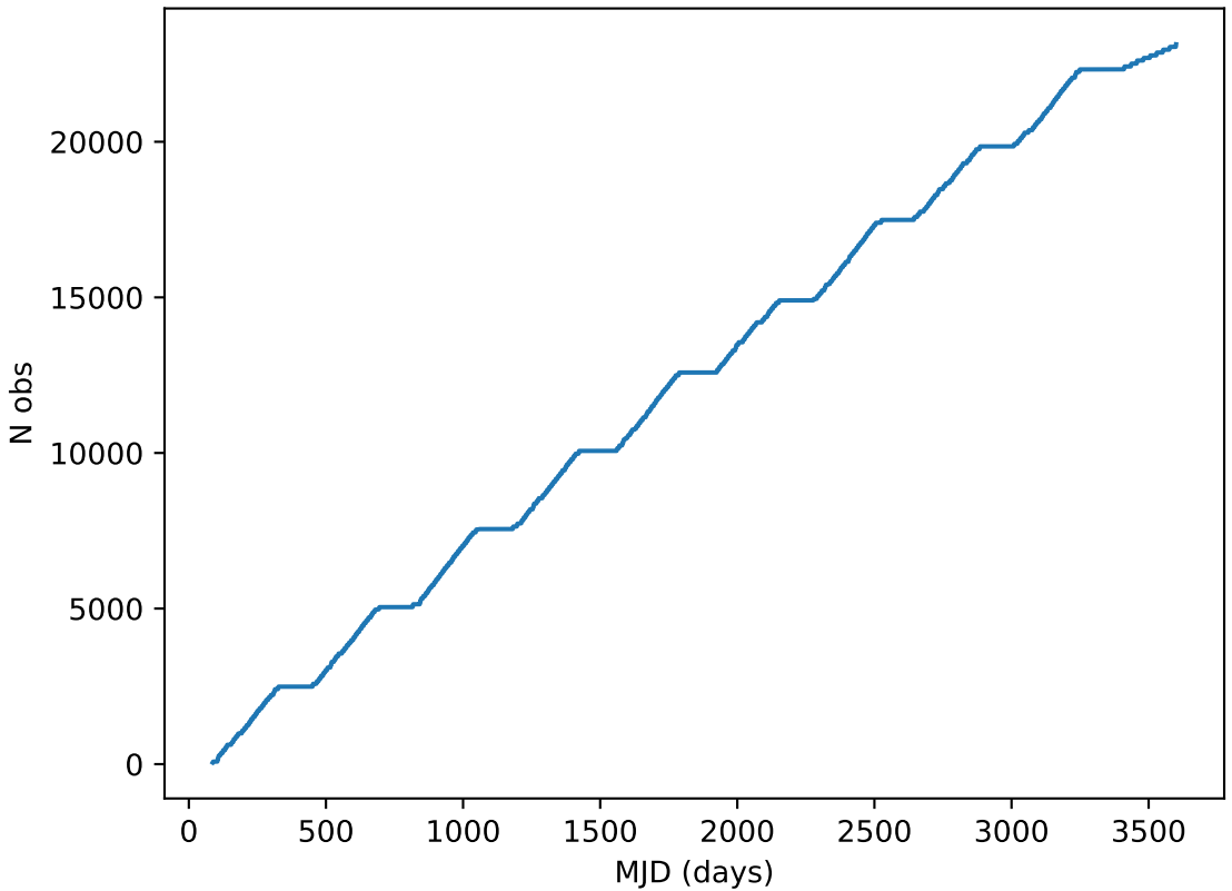
ddf_acor_sf15_lsf20_lsr50_v3.4_10yrs all bands: DD:EDFS Cumulative NVisits
