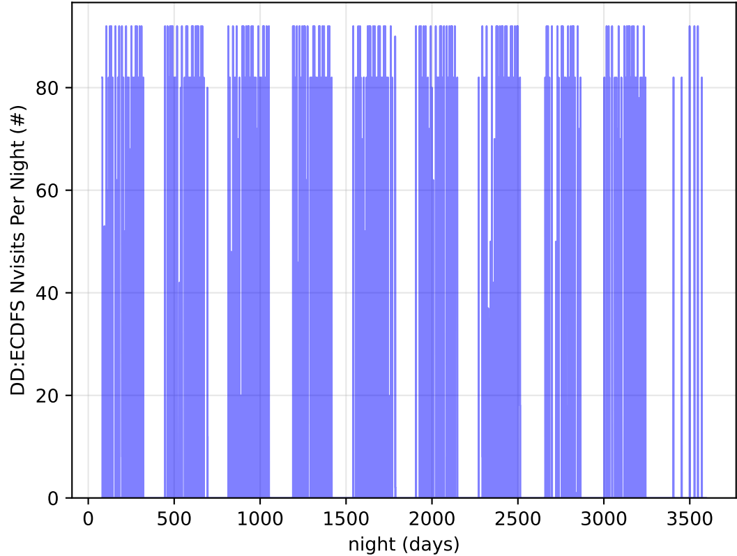
ddf_acor_sf15_lsf20_lsr50_v3.4_10yrs all bands: DD:ECDFS Nvisits Per Night
