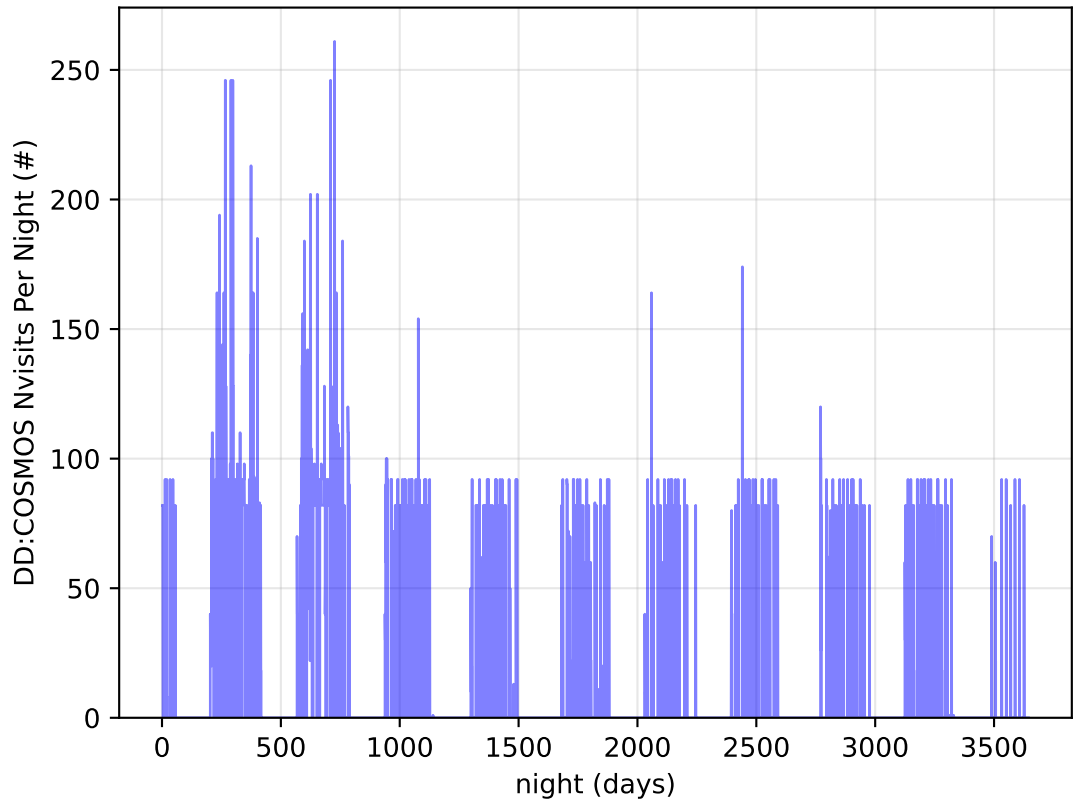
ddf_acor_sf15_lsf20_lsr50_v3.4_10yrs all bands: DD: COSMOS Nvisits Per Night
