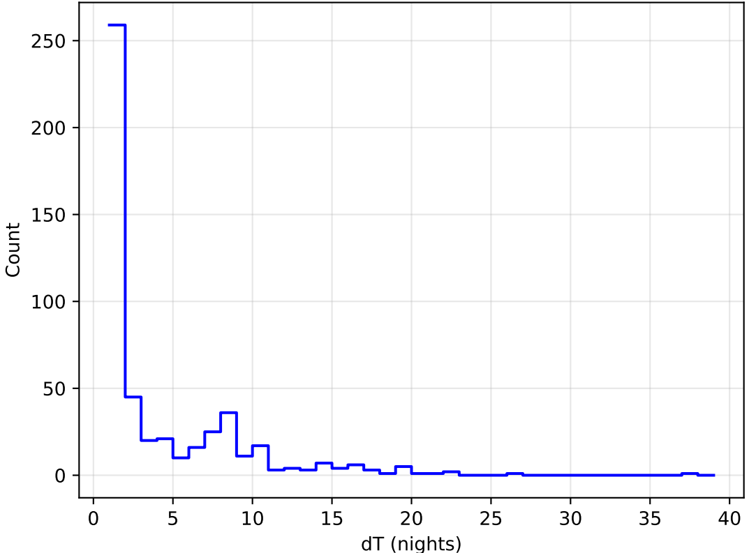
ddf_acor_sf15_lsf20_lsr50_v3.4_10yrs all bands: DD:COSMOS Delta Nights Histogram
