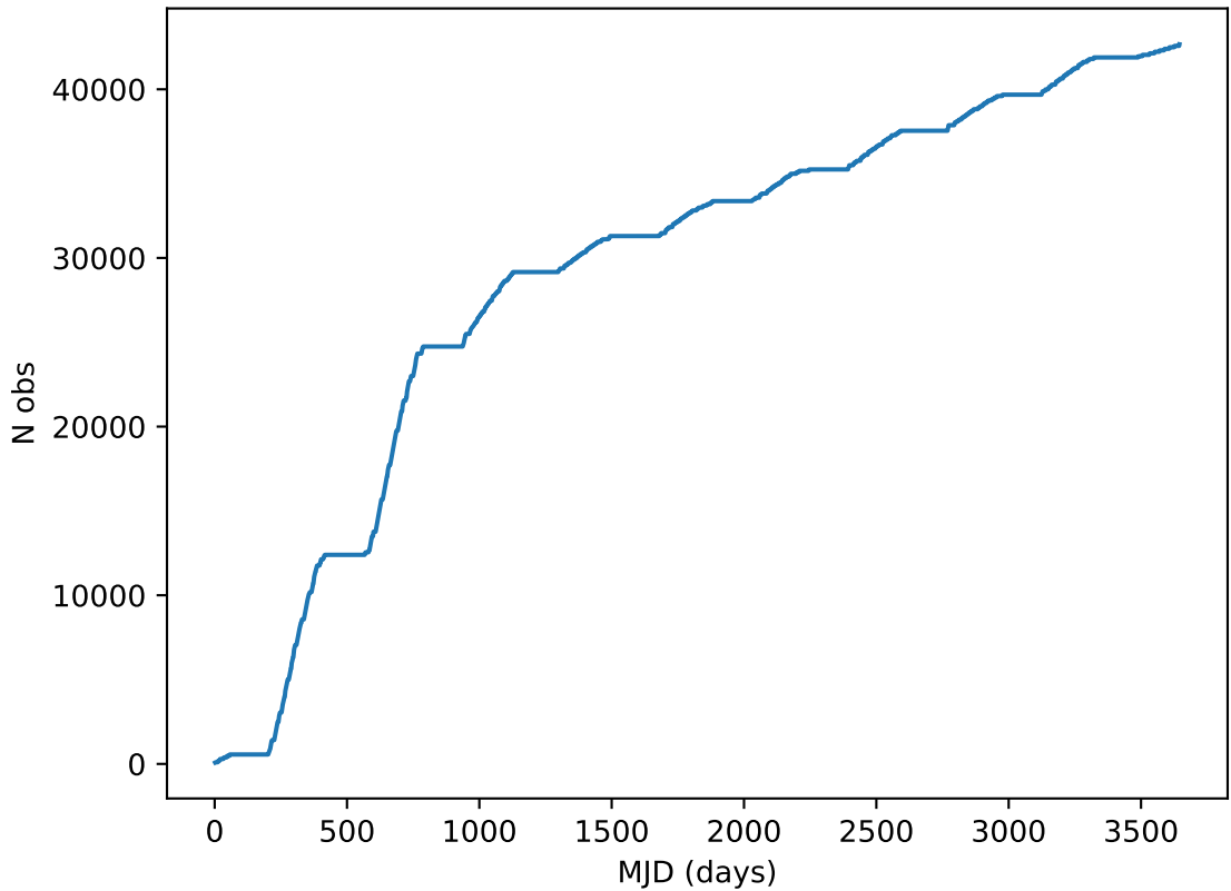
ddf_acor_sf15_lsf20_lsr50_v3.4_10yrs all bands: DD: COSMOS Cumulative NVisits
