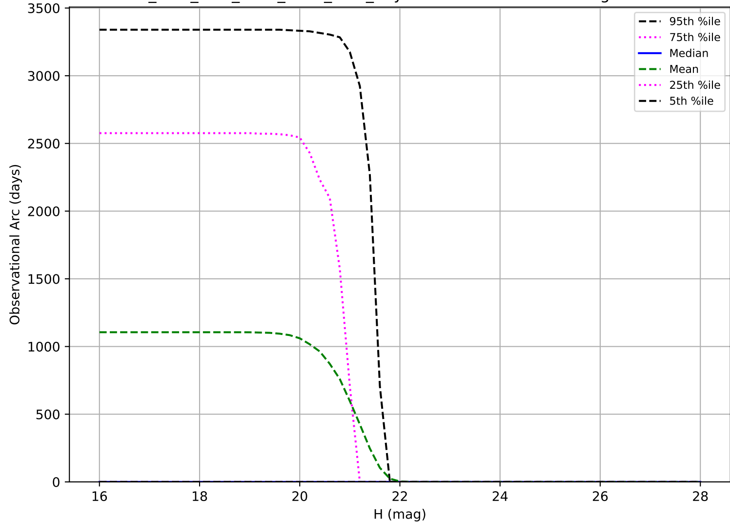
ddf_acor_sf15_lsf20_lsr20_v3.4_10yrs: Observational Arc Length Vatira
