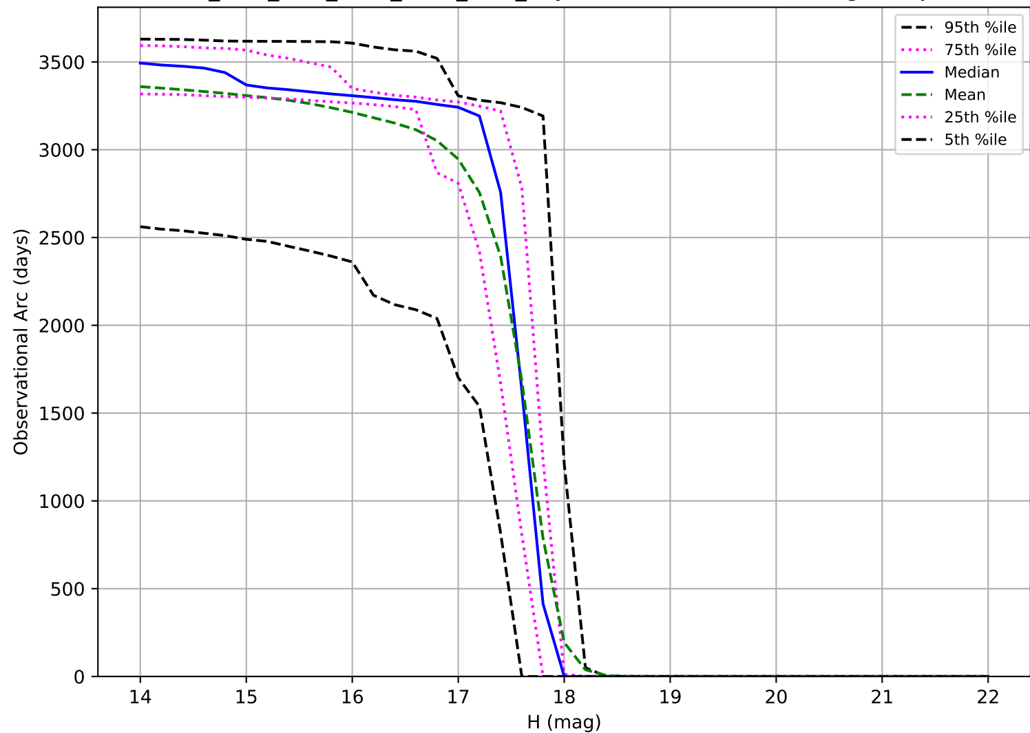
ddf_acor_sf15_lsf20_lsr20_v3.4_10yrs: Observational Arc Length Trojan
