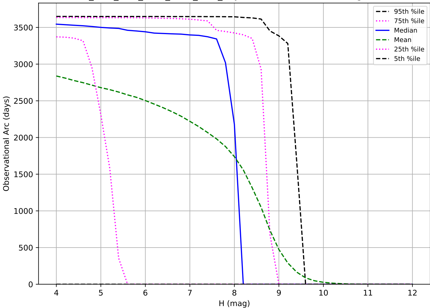
ddf_acor_sf15_lsf20_lsr20_v3.4_10yrs: Observational Arc Length TNO
