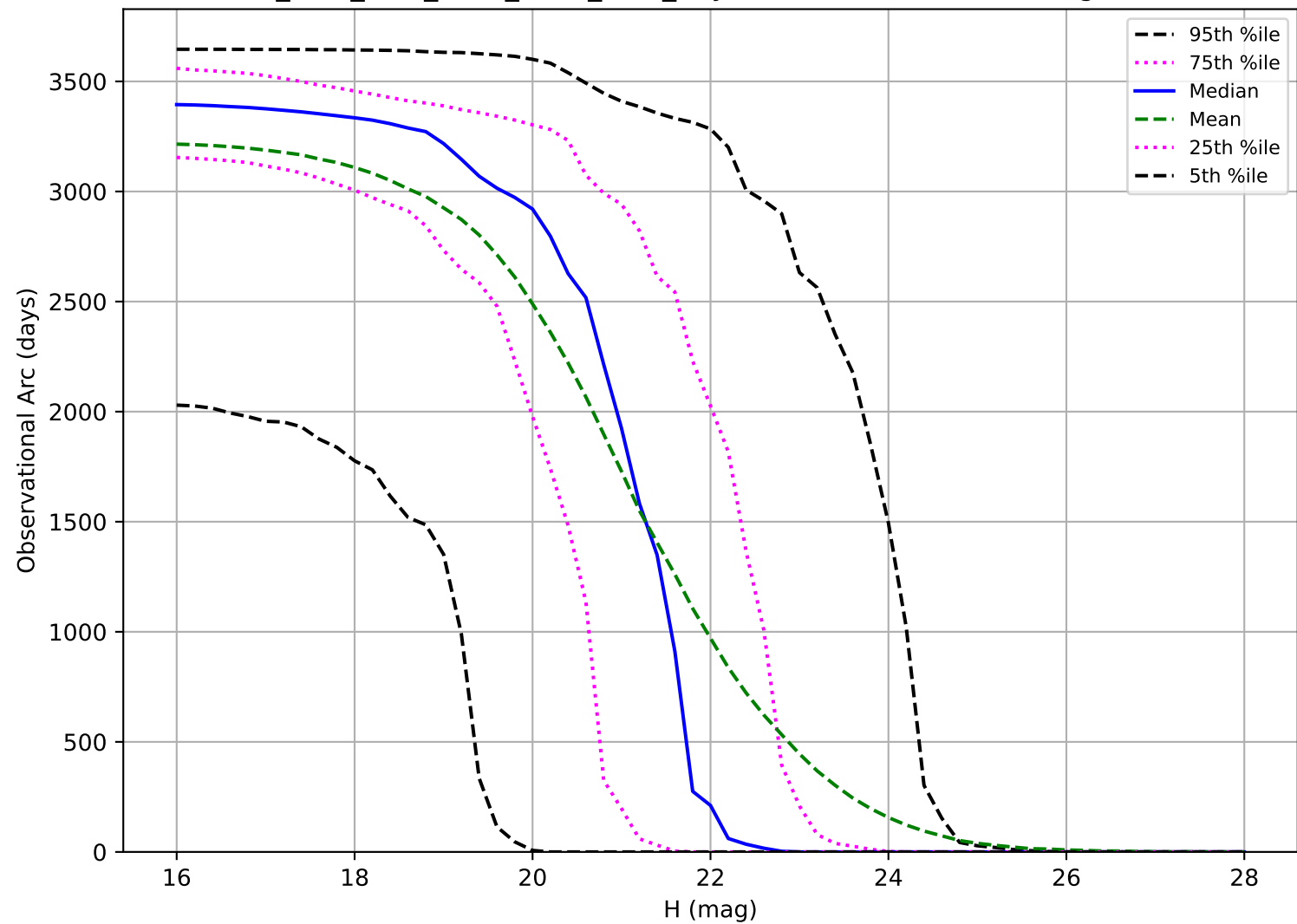
ddf_acor_sf15_lsf20_lsr20_v3.4_10yrs: Observational Arc Length PHA
