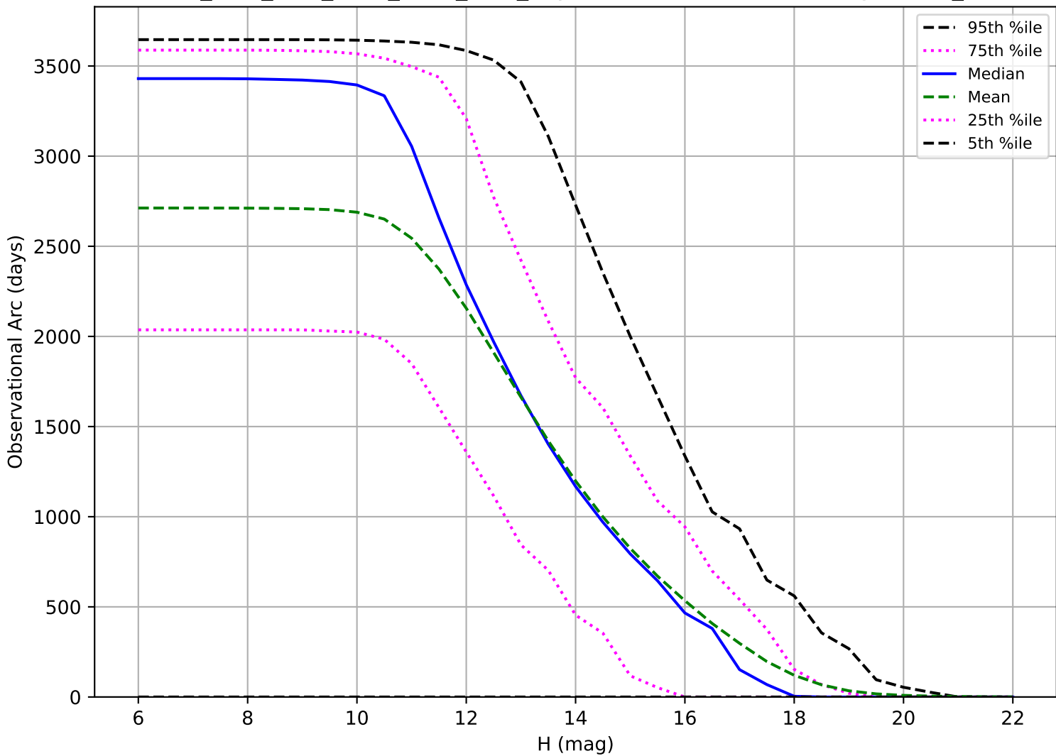
ddf_acor_sf15_lsf20_lsr20_v3.4_10yrs: Observational Arc Length OCC_r5
