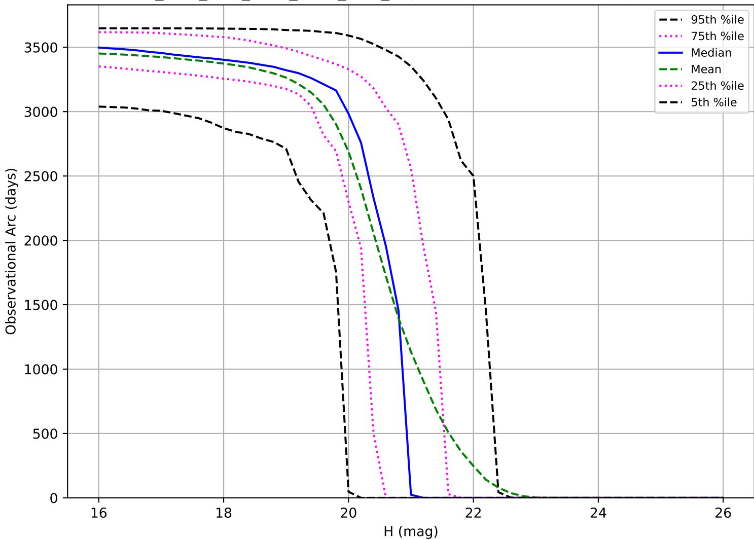
ddf_acor_sf15_lsf20_lsr20_v3.4_10yrs: Observational Arc Length MBA
