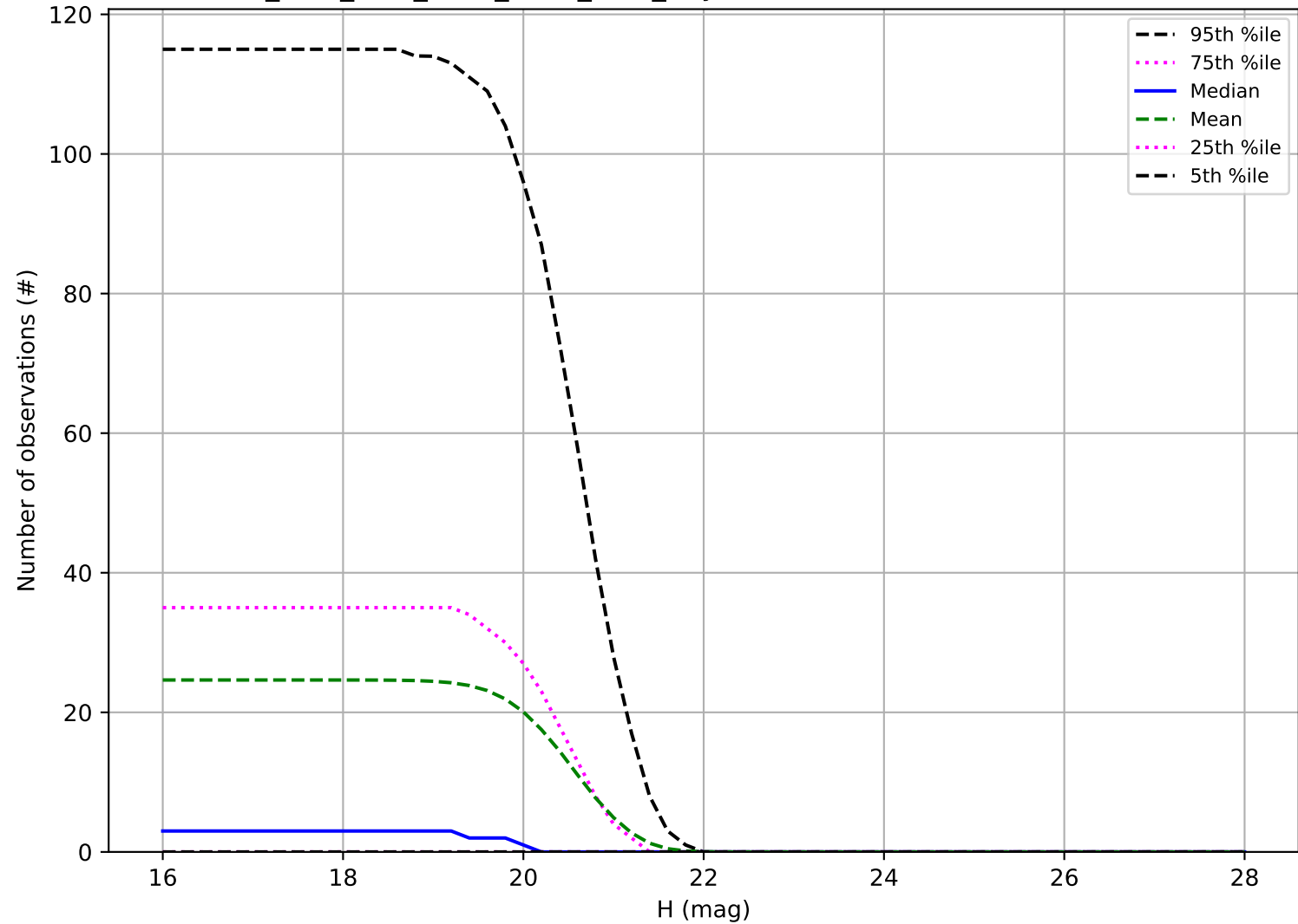
ddf_acor_sf15_lsf20_lsr20_v3.4_10yrs: Number of observations Vatira
