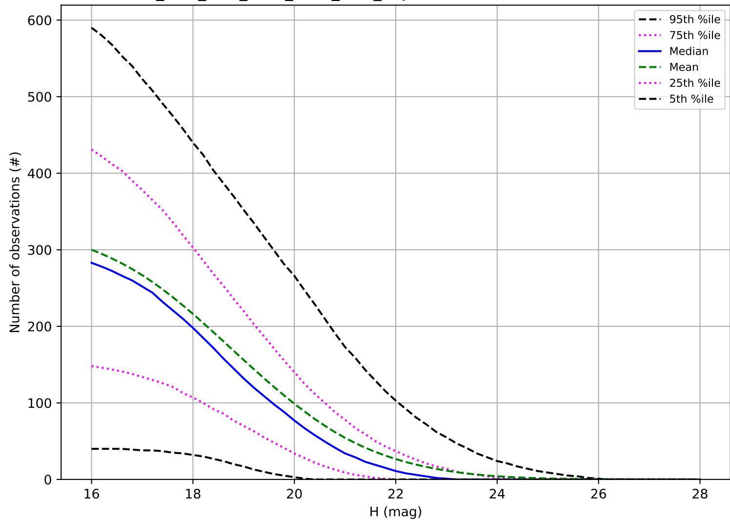
ddf_acor_sf15_lsf20_lsr20_v3.4_10yrs: Number of observations PHA
