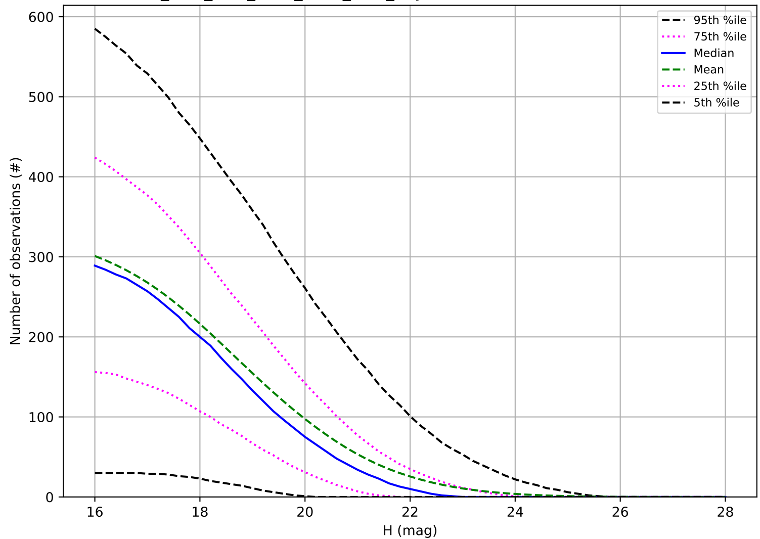
ddf_acor_sf15_lsf20_lsr20_v3.4_10yrs: Number of observations NEO
