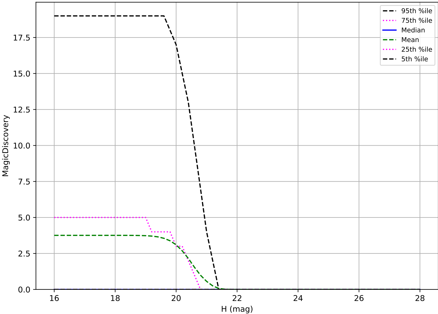
ddf_acor_sf15_lsf20_lsr20_v3.4_10yrs: Vatira 6 detections in 60 nights detection loss
