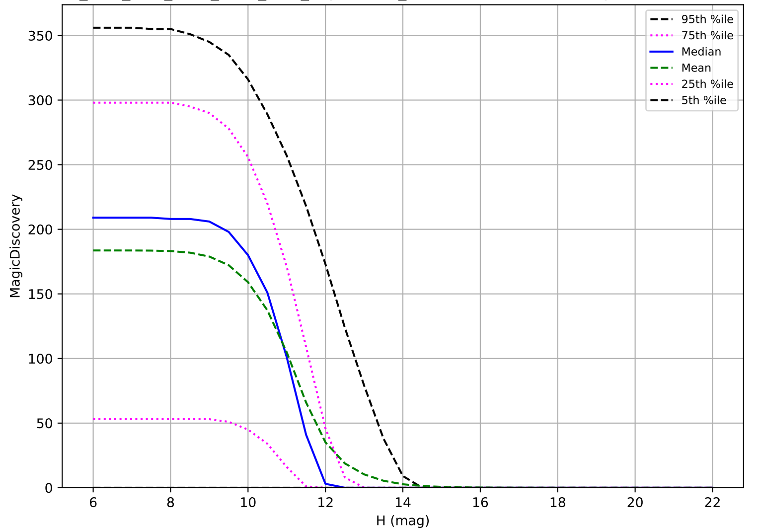
ddf_acor_sf15_lsf20_lsr20_v3.4_10yrs: OCC_r20 6 detections in 60 nights detection loss
