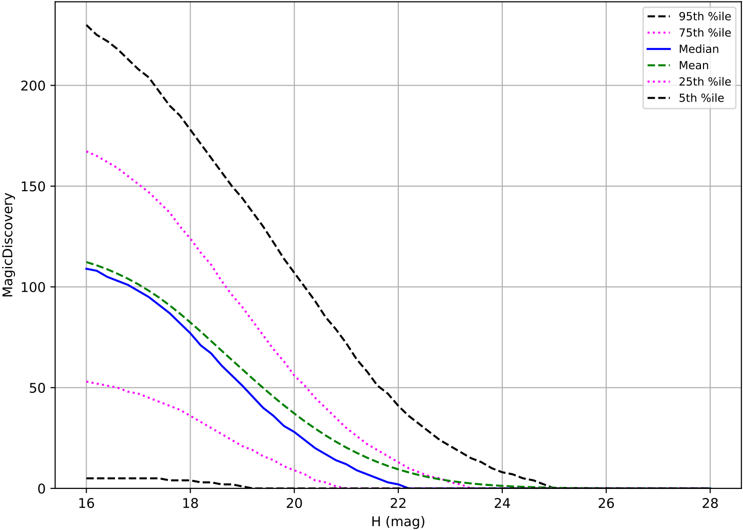
ddf_acor_sf15_lsf20_lsr20_v3.4_10yrs: NEO 6 detections in 60 nights detection loss
