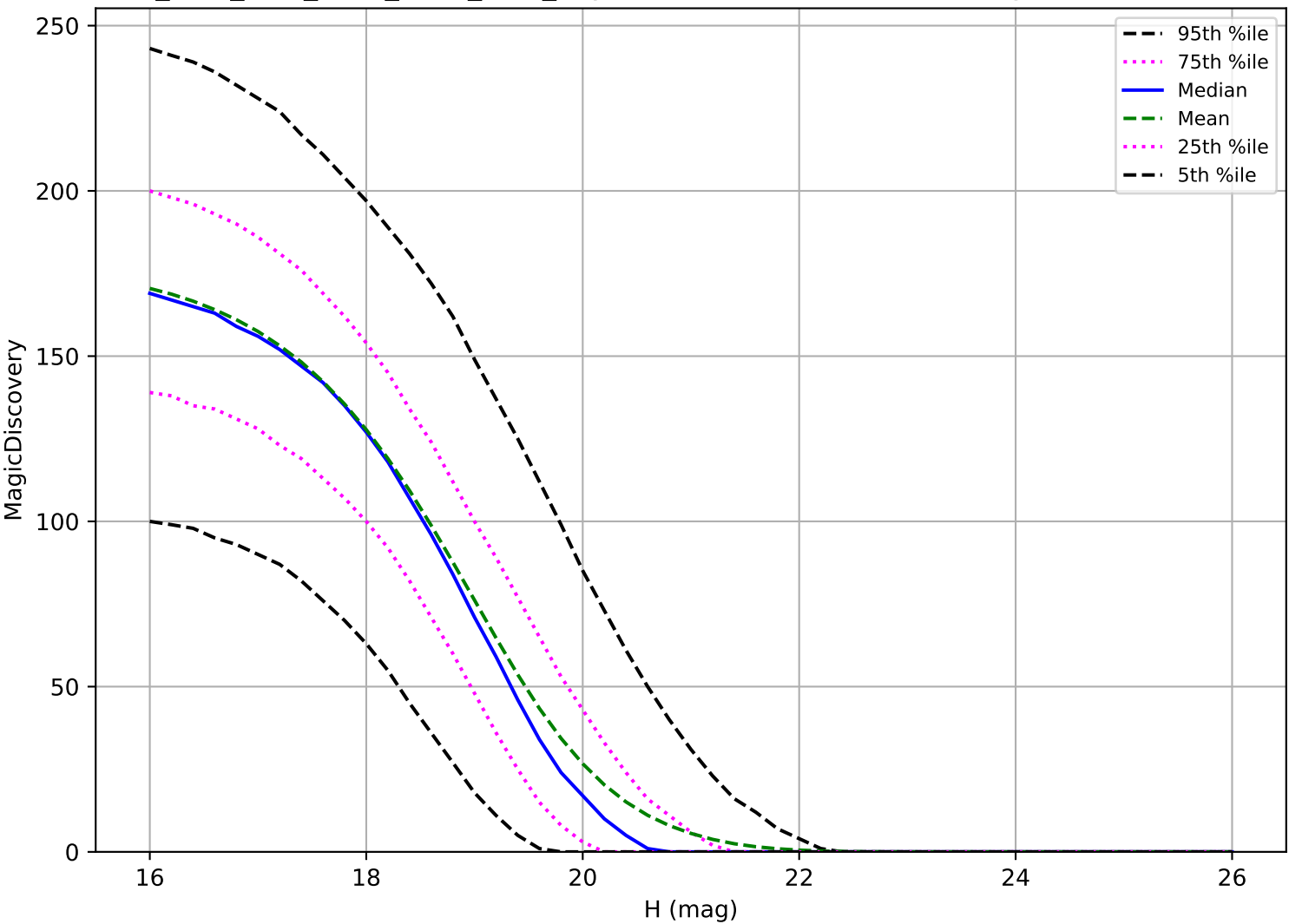
ddf_acor_sf15_lsf20_lsr20_v3.4_10yrs: MBA 6 detections in 60 nights detection loss
