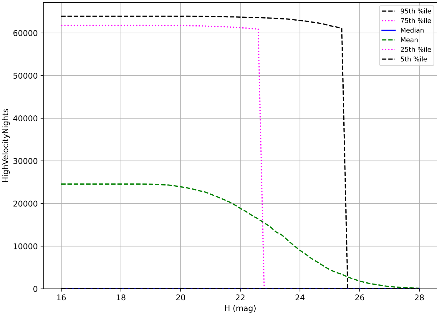
ddf_acor_sf15_lsf20_lsr20_v3.4_10yrs: PHA High velocity pair detection loss
