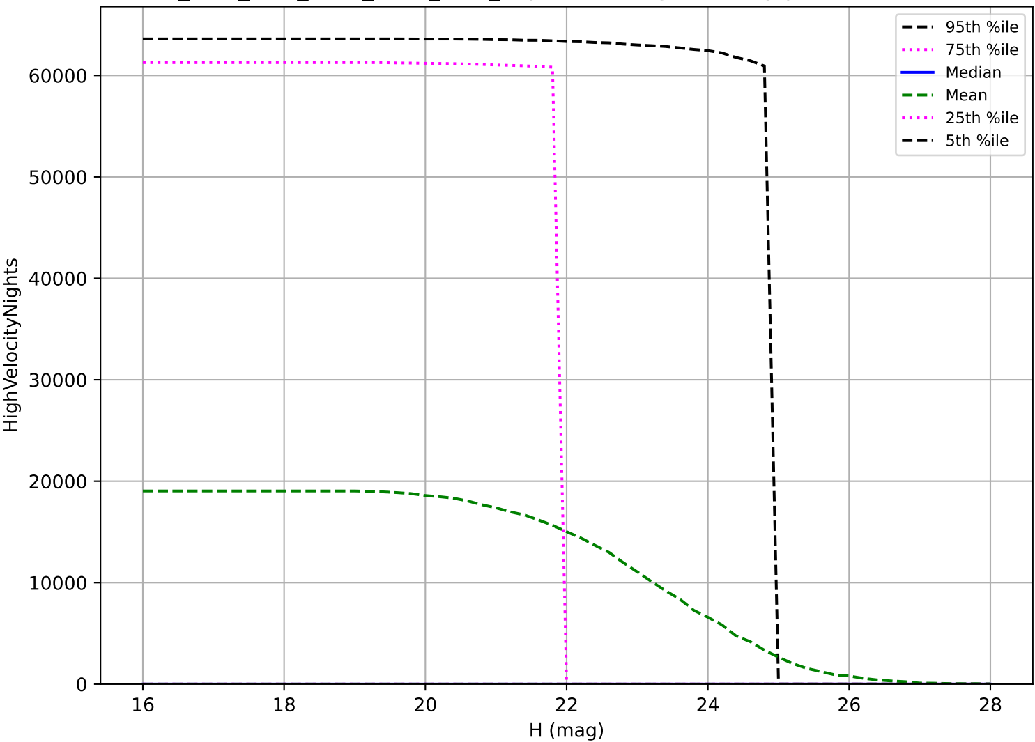
ddf_acor_sf15_lsf20_lsr20_v3.4_10yrs: NEO High velocity pair detection loss
