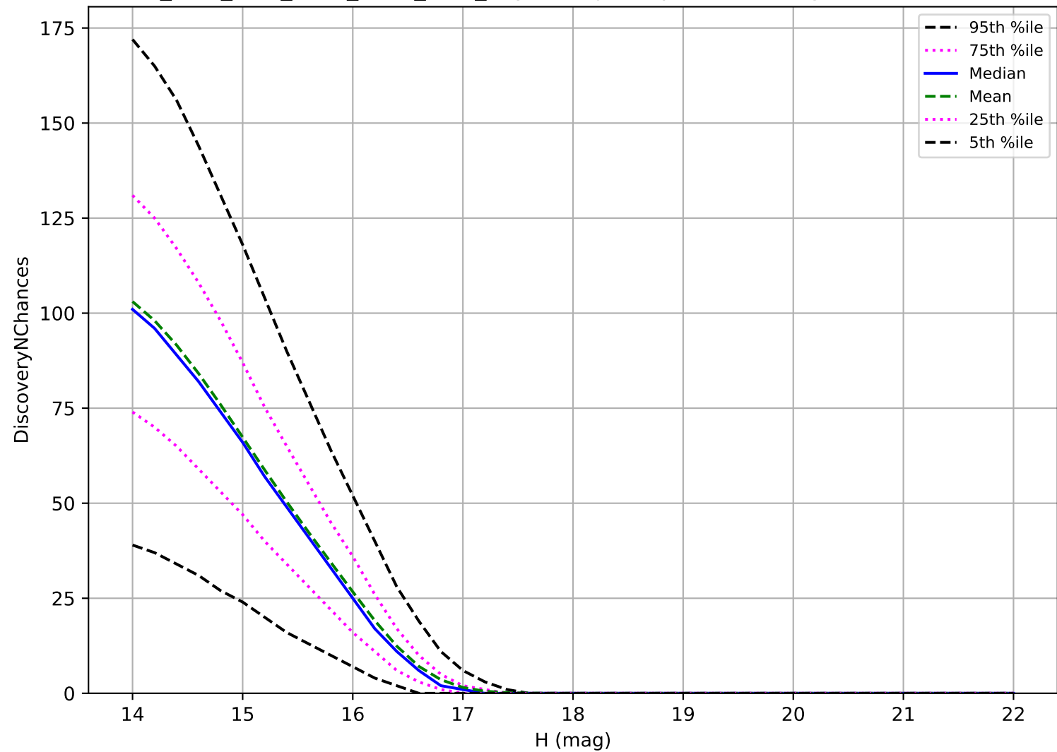
ddf_acor_sf15_lsf20_lsr20_v3.4_10yrs: Trojan 3 pairs in 15 nights detection loss
