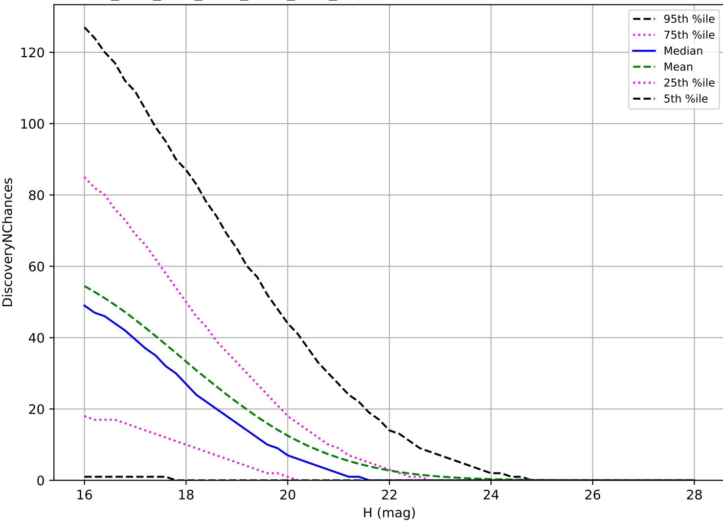
ddf_acor_sf15_lsf20_lsr20_v3.4_10yrs: PHA 3 pairs in 15 nights detection loss
