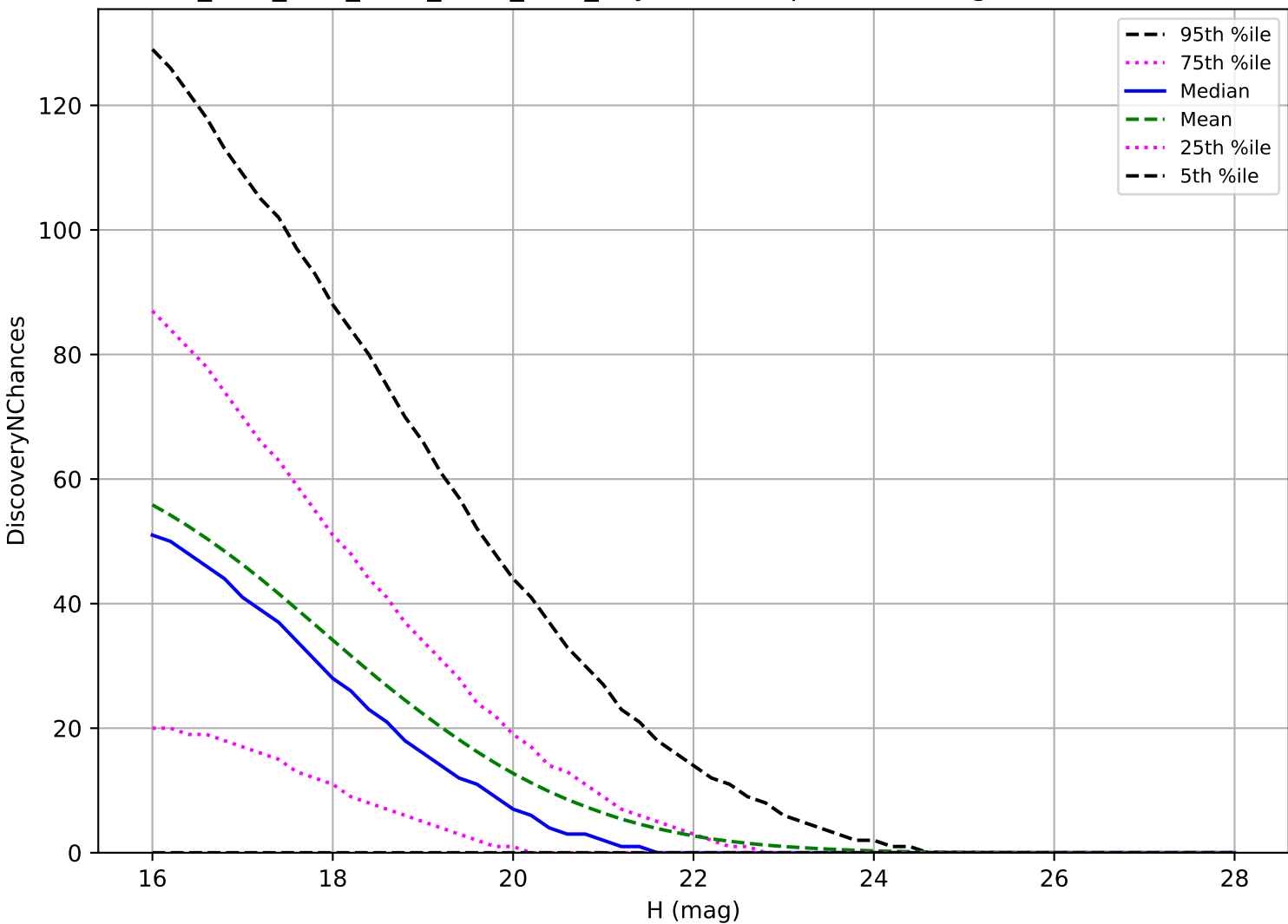
ddf_acor_sf15_lsf20_lsr20_v3.4_10yrs: NEO 3 pairs in 15 nights detection loss
