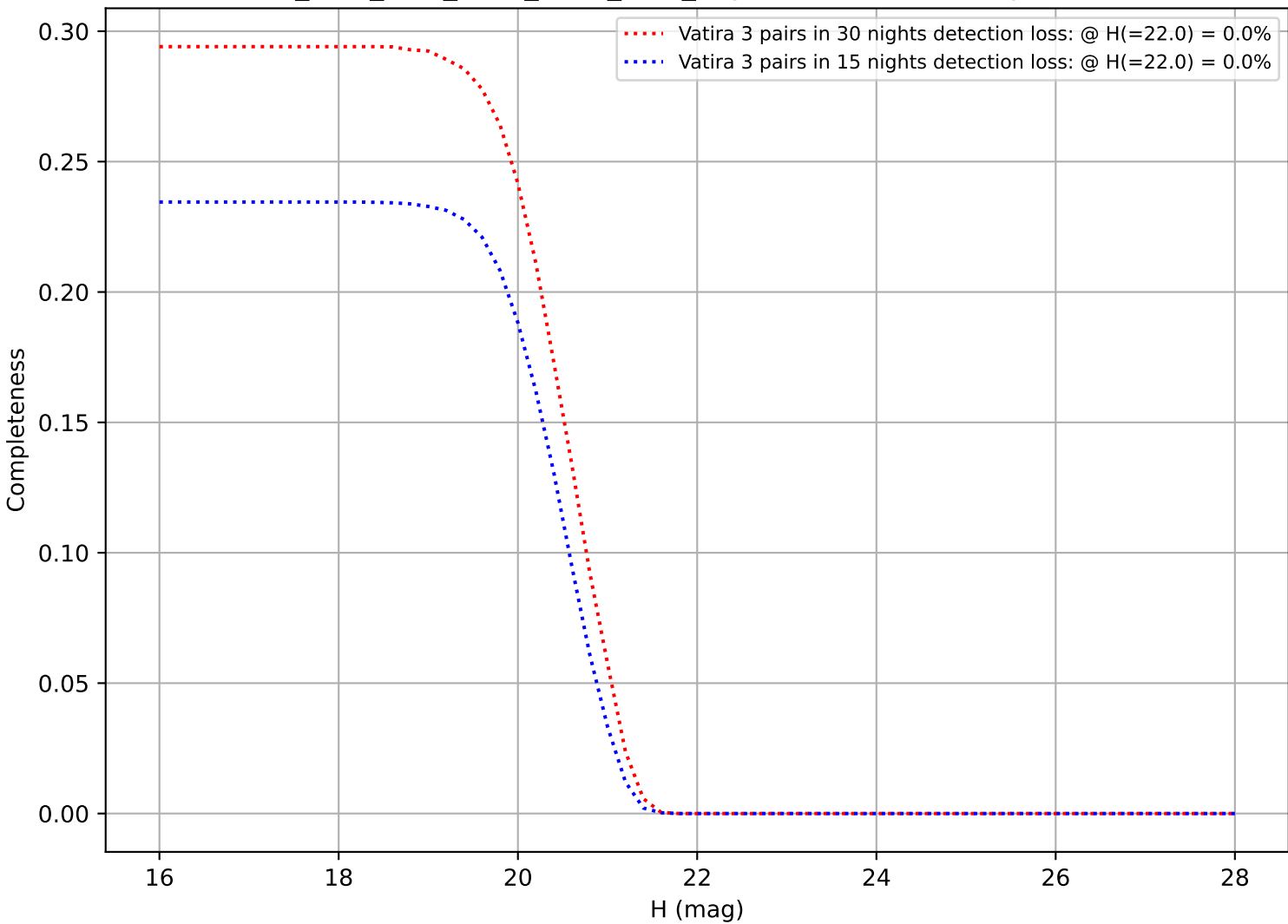
ddf_acor_sf15_lsf20_lsr20_v3.4_10yrs: DifferentialCompleteness
