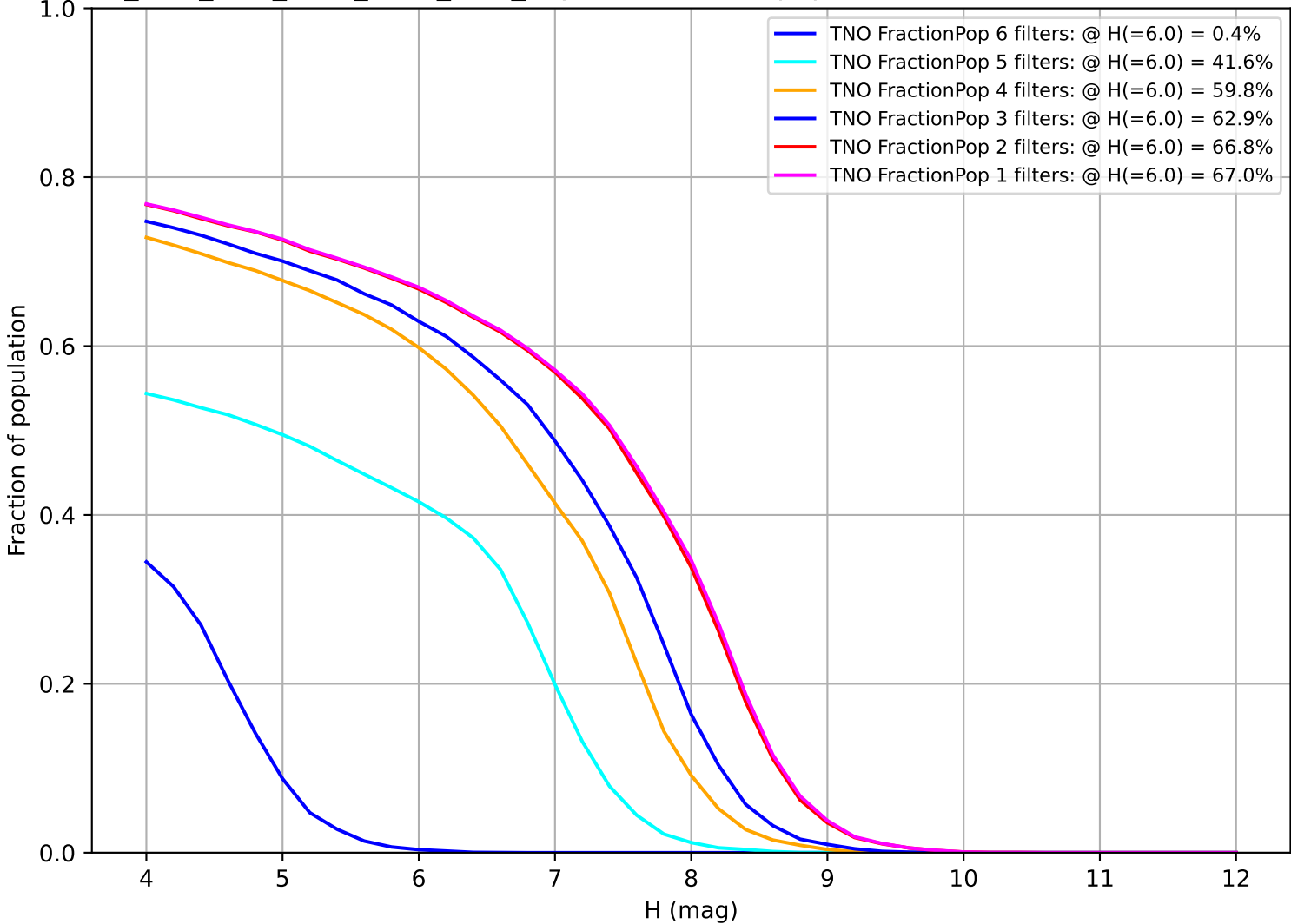
ddf_acor_sf15_lsf20_lsr20_v3.4_10yrs: Fraction of population with colors in X filters TNO
