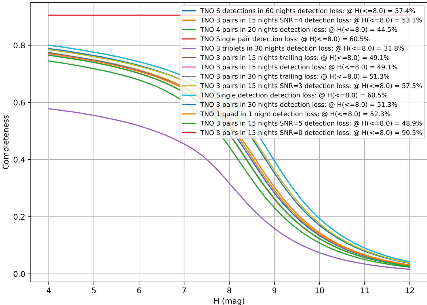
ddf_acor_sf15_lsf20_lsr20_v3.4_10yrs: CumulativeCompleteness
