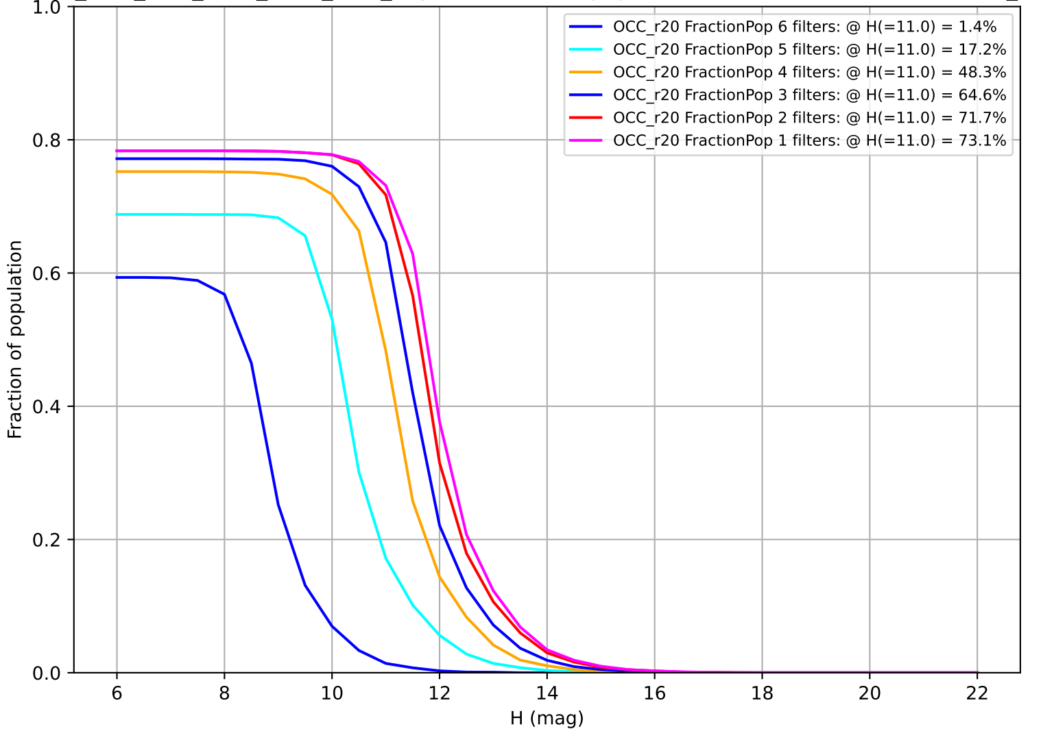
ddf_acor_sf15_lsf20_lsr20_v3.4_10yrs: Fraction of population with colors in X filters OCC_r20
