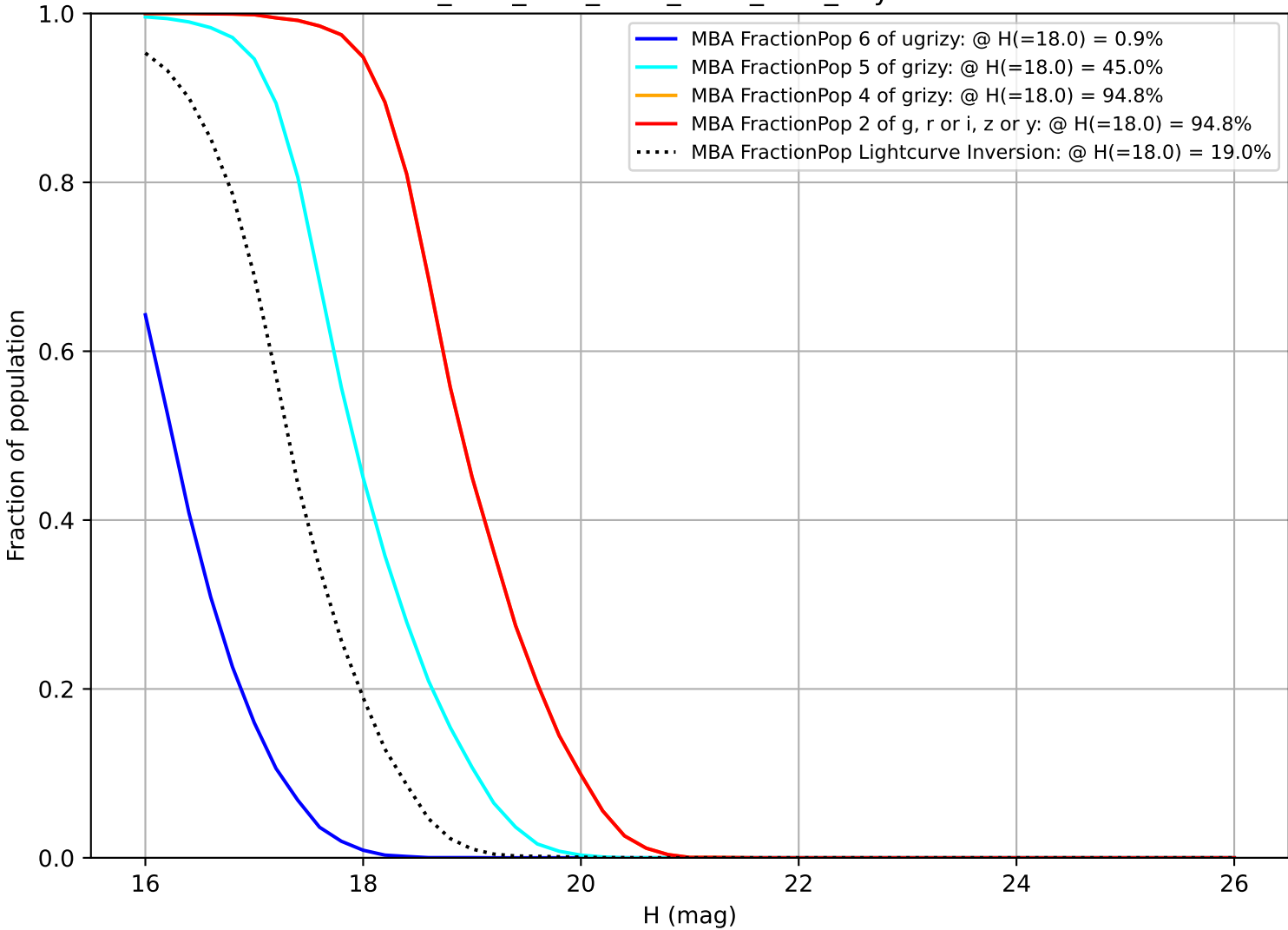
ddf_acor_sf15_lsf20_lsr20_v3.4_10yrs MBA
