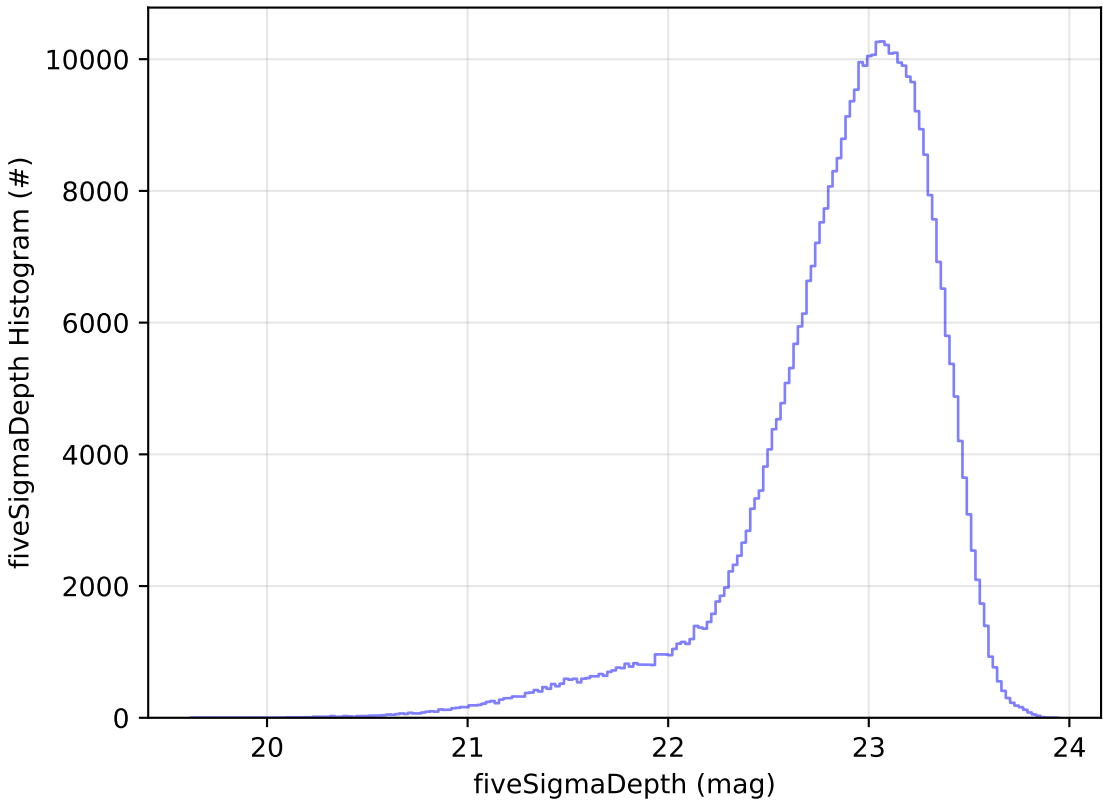
ddf_acor_sf15_lsf20_lsr20_v3.4_10yrs z: fiveSigmaDepth Histogram
