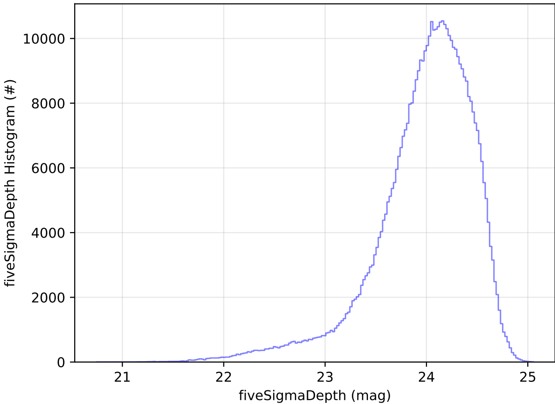
ddf_acor_sf15_lsf20_lsr20_v3.4_10yrs r: fiveSigmaDepth Histogram
