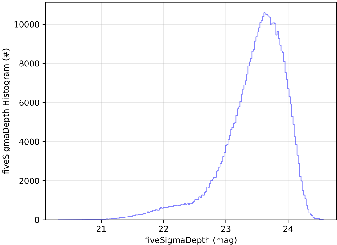
ddf_acor_sf15_lsf20_lsr20_v3.4_10yrs i: fiveSigmaDepth Histogram
