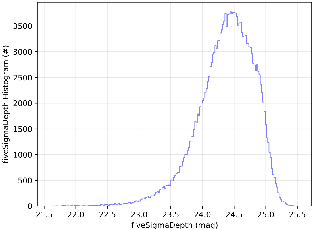
ddf_acor_sf15_lsf20_lsr20_v3.4_10yrs g: fiveSigmaDepth Histogram
